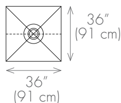
STC-TRAY91/91
