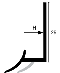
Section PVC
